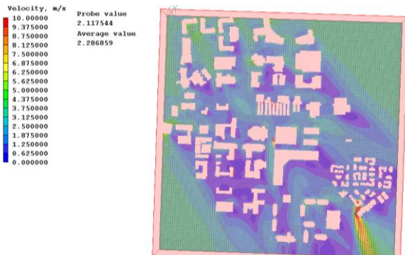
Figure 2. Plane velocity of the outdoor airflow on campus
