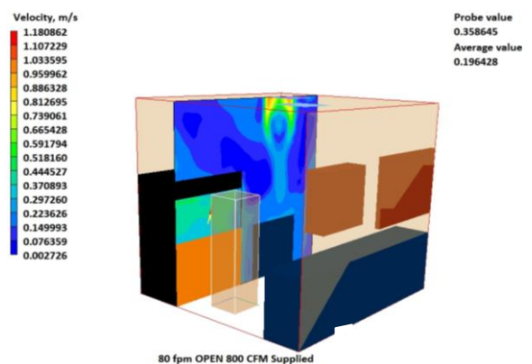
Figure 1: Simulated results for 80 fpm (0.4 m/s) face velocity with 800 cfm tracer gas
